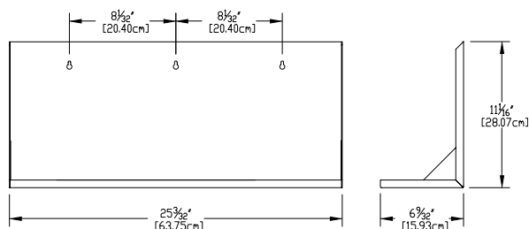
Part Number 440.0625 C Cabinet
