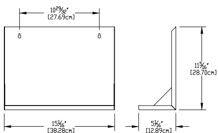
Part Number 440.0616 A Cabinet
