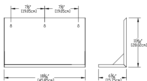
Part Number 440.0620 B Cabinet
