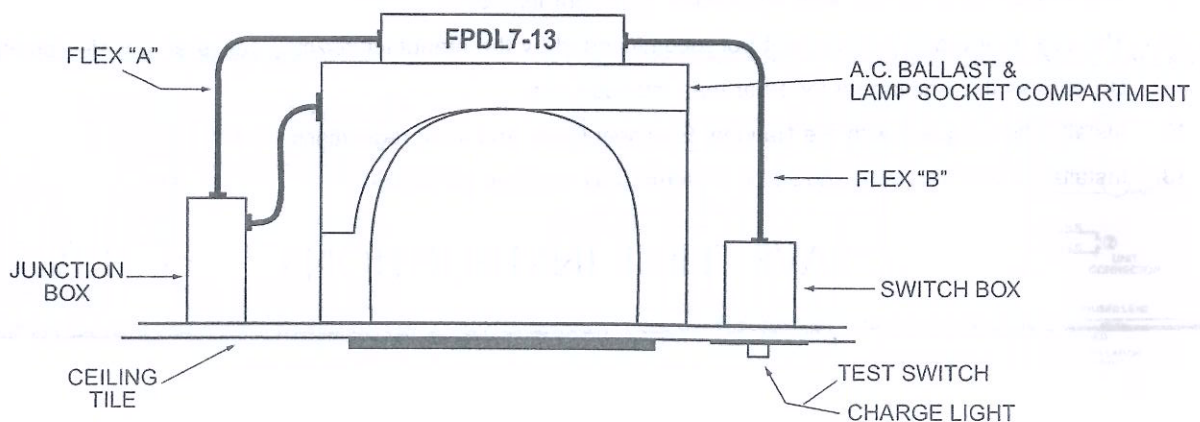
Illustration 1 Downlight Fixture
