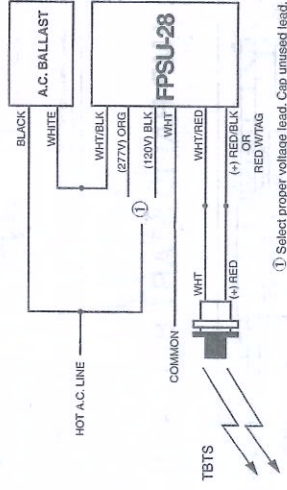
Unswitched Fixture
