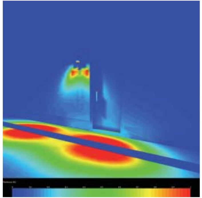
3D light level colored scale of 0 to 1 foot-candle of Literay in the new exterior application standard.
