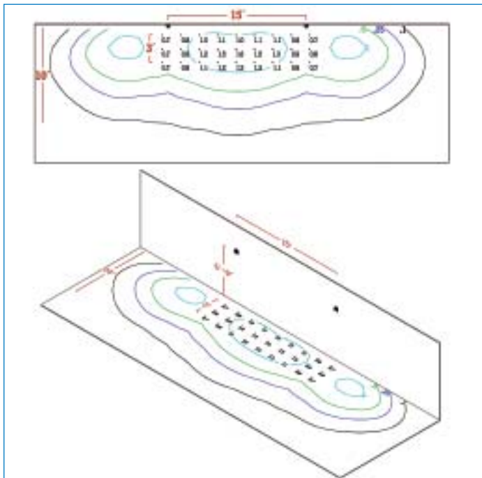
ISO Curve on a point-by-point grid of 2 Literay luminaries.
