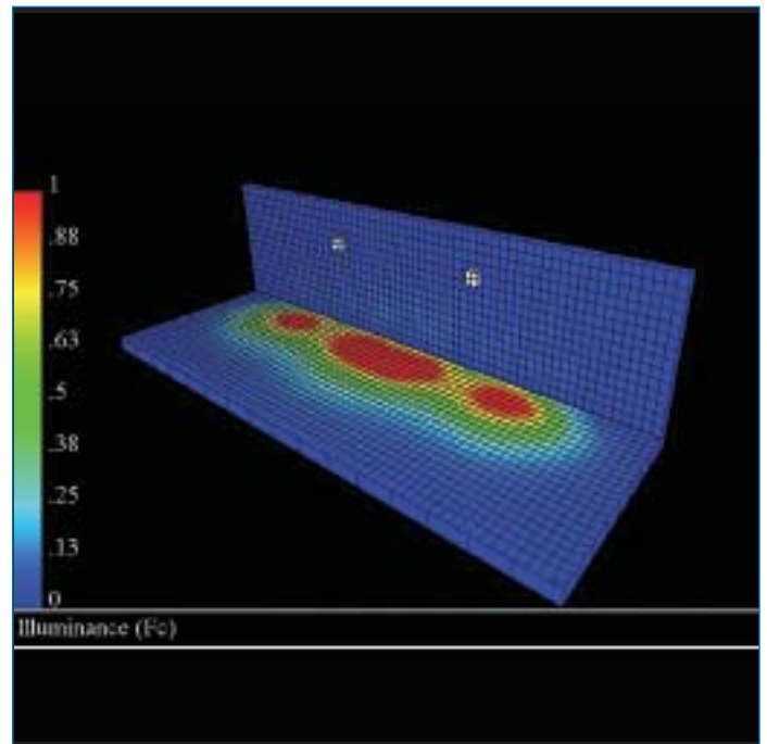
3D light level colored scale of 0 to 1 foot-candle of two Literay luminaries.
