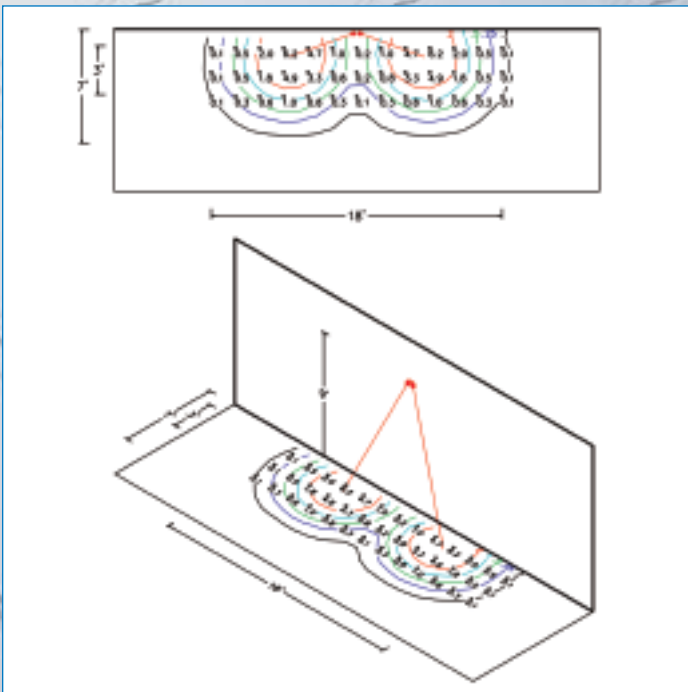
ISO CURVE ON A POINT-BY-POINT GRID OF A SINGLE SURVIVE-ALL™ SVX SERIES COMBO UNIT
