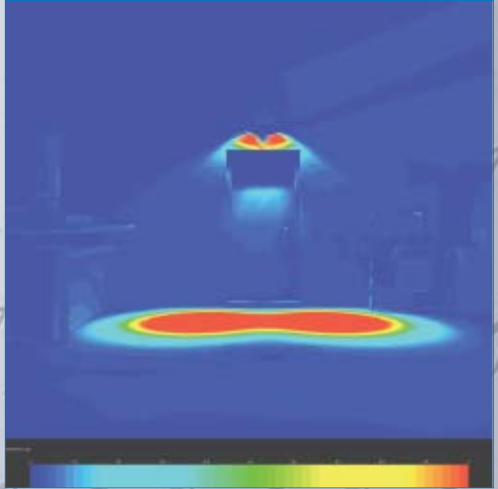
3D LIGHT LEVEL COLORED SCALE IMAGE OF 0 TO 1 FOOT - CANDLE OF THE SURVIVE-ALL™ UNIT
