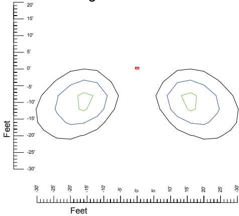
Mounting at 20'
