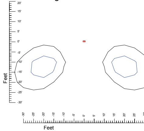
Mounting at 25'
