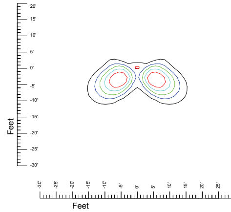
Mounting at 15'
