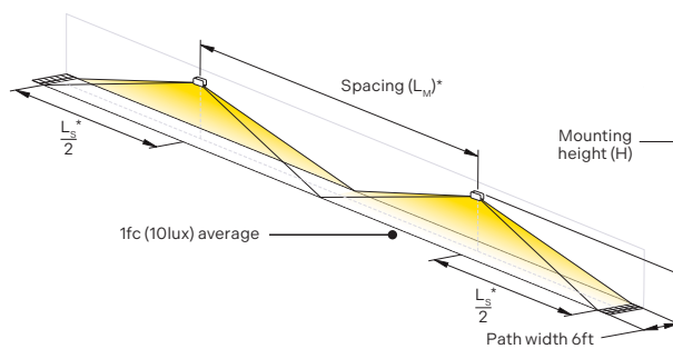
Multiple luminaires-Fig. 3 (Continuous hallway)
