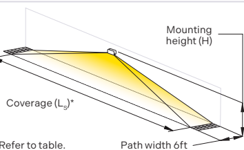
Single luminaire-Fig. 1 (Coverage in opposite directions with no subsequent luminaire)
