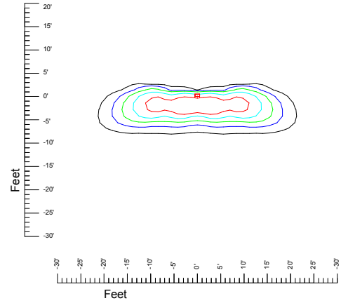
Mounting at 15'
