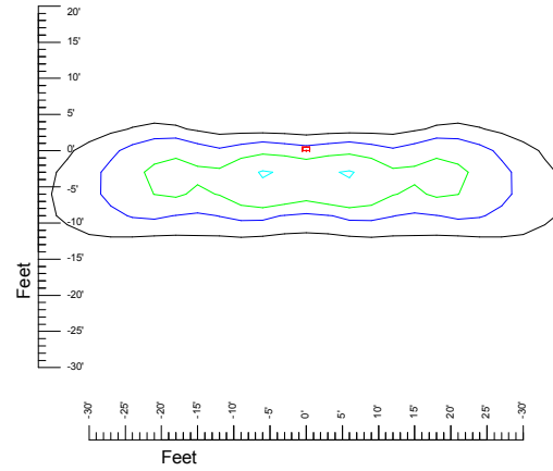
Mounting at 15'
